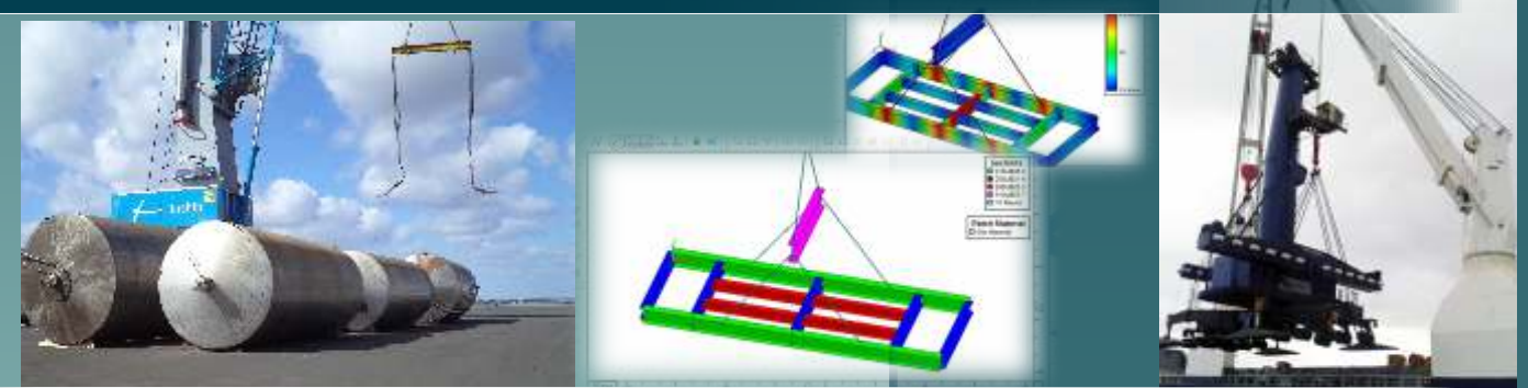
Calculations of heavy lift maneuvers: Design of lifting beams.
